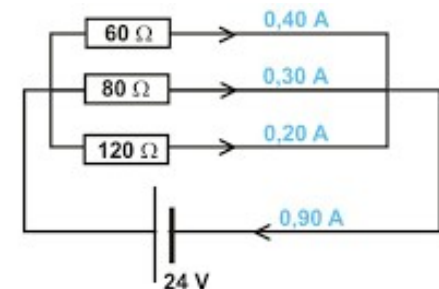
Parallel schakeling
